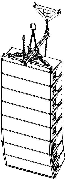
KSL8/KSL12 Line-Array 8-tief, Compression Mode Setup - Vorderansicht
