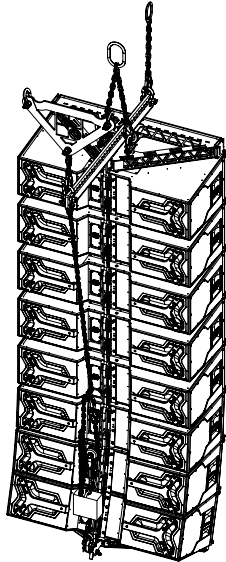
KSL8/KSL12 Line-Array 8-tief, Compression Mode Setup - Rückansicht
