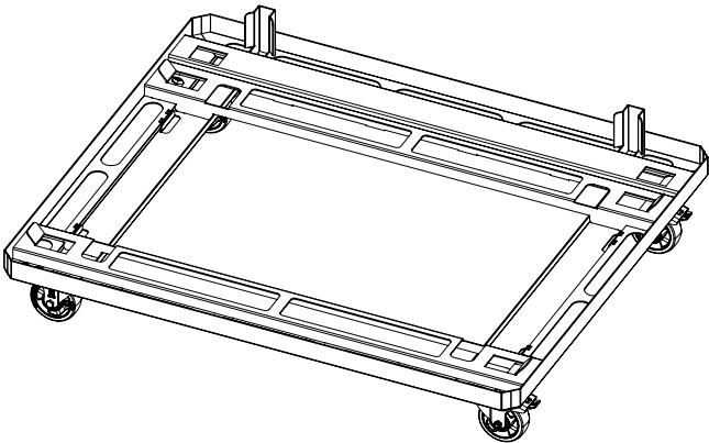
E7492 Touring Cart SL-SUB/SL-GSUB
