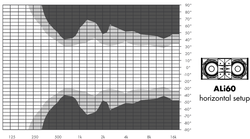
ALi60 horizontal isobars
