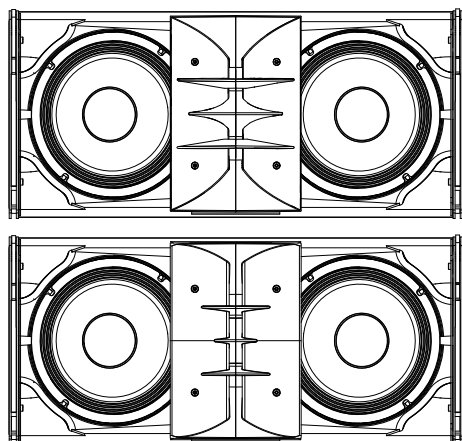
ALi60/ALi90 loudspeaker
