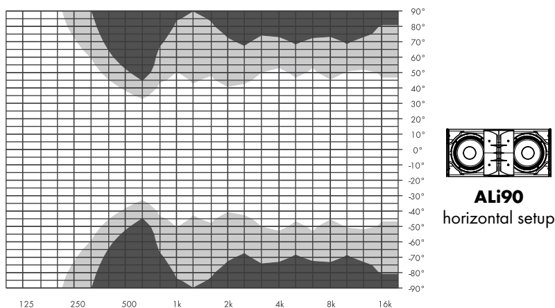
ALi90 horizontal isobars
