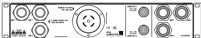
Z5566.001 Rear panel
