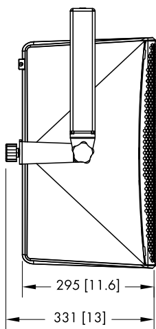
Z5803 Einbaumaße in mm [Zoll]
