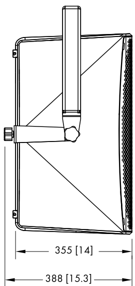
Z5806 Einbaumaße in mm [Zoll]
