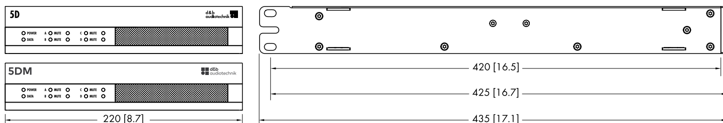
5D/5DM enclosure dimensions in mm [inch]
