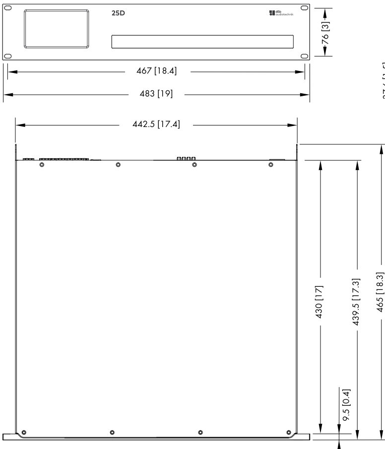
25D enclosure dimensions in mm [inch]
