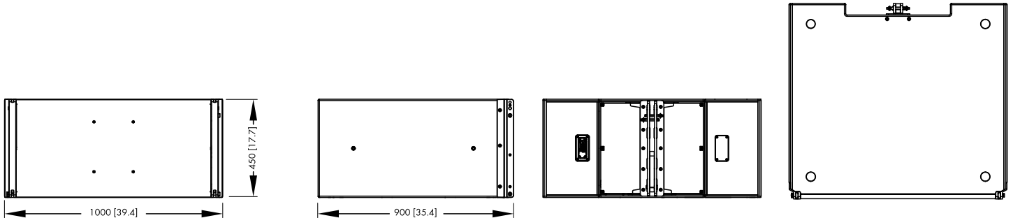
KSLi-SUB cabinet dimensions in mm [inch]
