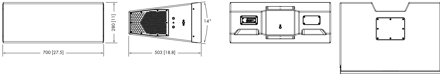
XSLi12 SVS cabinet dimensions in mm [inch]
