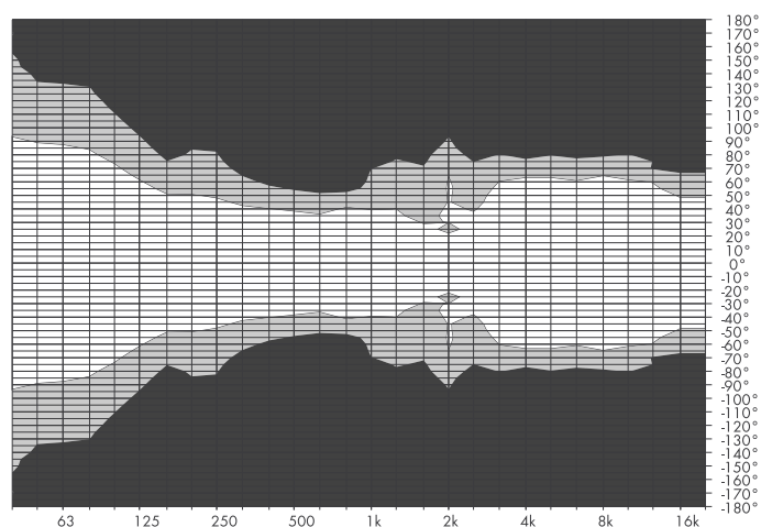
Diagramme isobare horizontal KSL12
