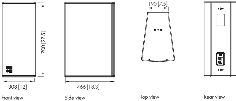
Vi10P cabinet dimensions in mm [inch]
