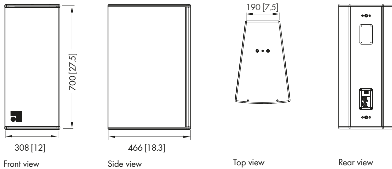
Vi7P cabinet dimensions in mm [inch]
