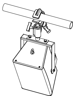
Fig. 1: 8S loudspeaker
