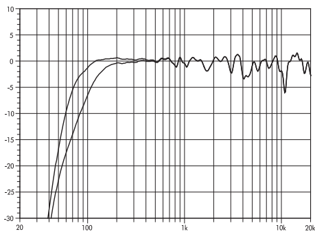
Fig. 9: 8S frequency response, standard and CUT modes
