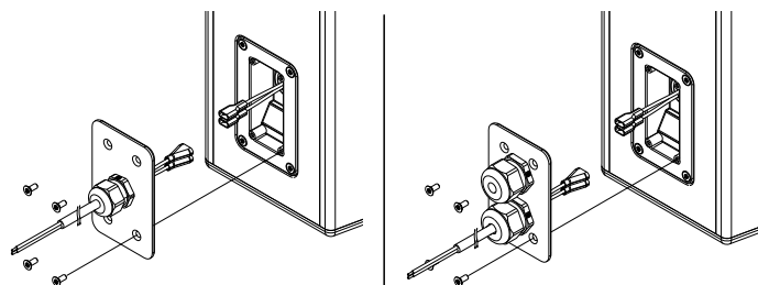
Faston-Type-Anschluss, männlich, 1 x PG (standard), 2 x PG (optional)
