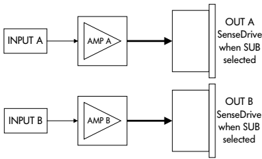
D12 Input/Output Routing "Dual Channel"
