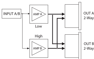
D12 Input/Output Routing "2-Way Active"
