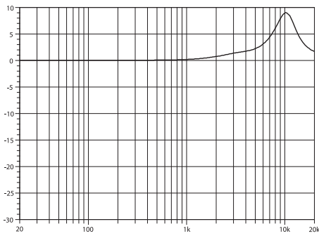
Fig. 4: Frequency response correction of HFC circuit
