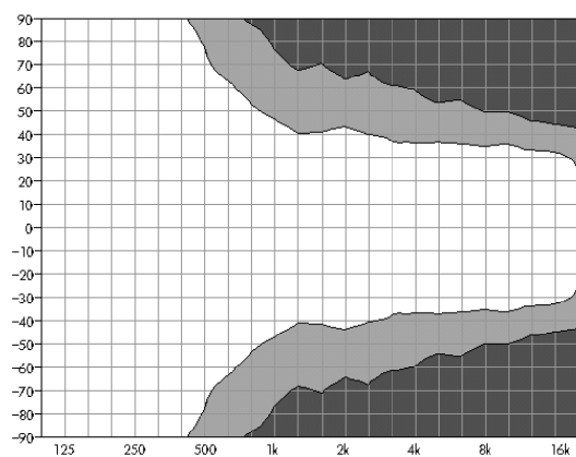
Fig. 5: Diagramme isobare Qi7 horizontal, configuration standard
