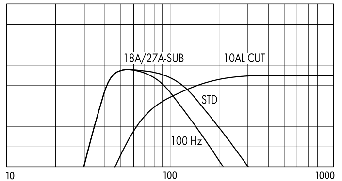
10AL / 18A/27A-SUB crossover setup
